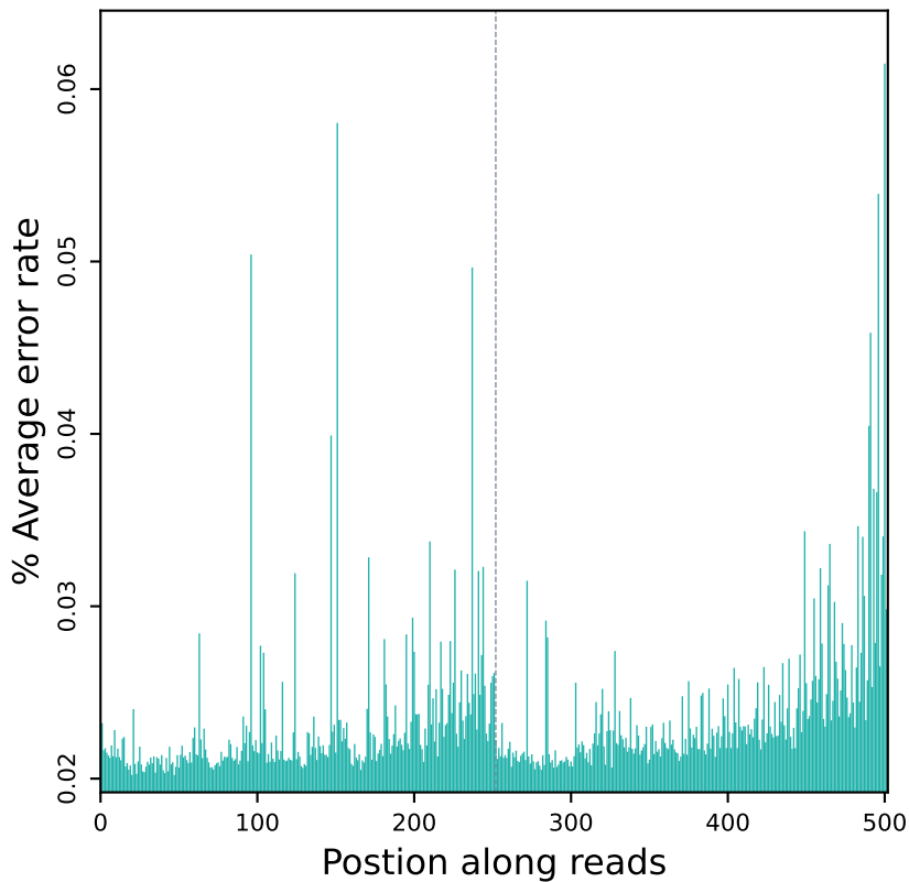
Error rate distribution along reads (R10528)
